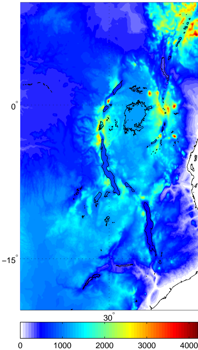
Elevation (m)
